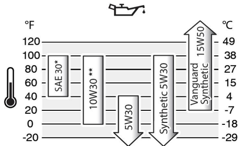
SAE Viscosity Grades
