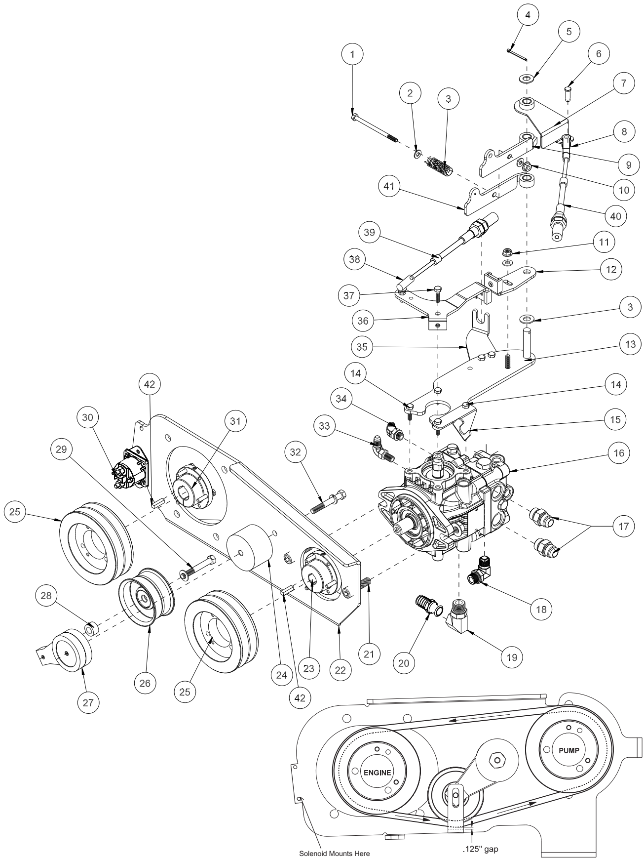
Belt Routing
