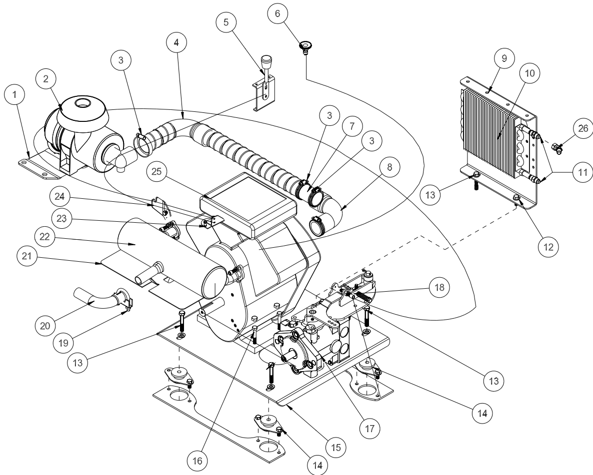
Cyclonic air cleaner 42-834
