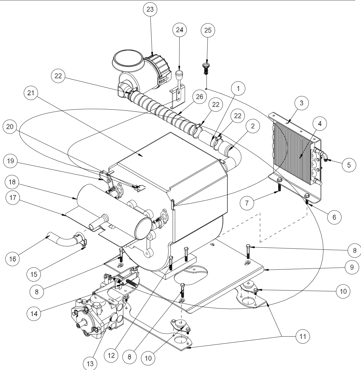
Cyclonic air cleaner 42-834
