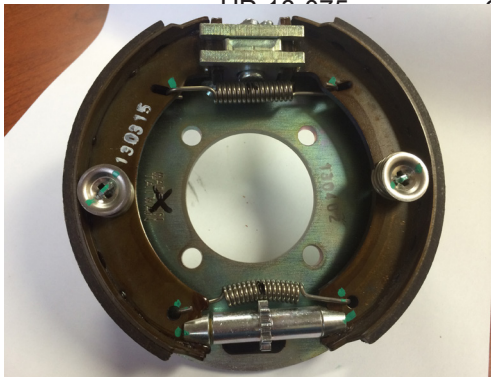
43-241-01 Brake Assembly
